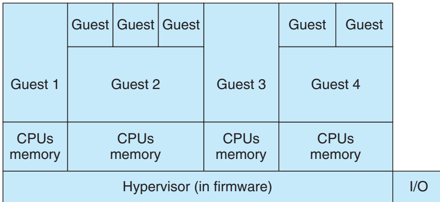
Figure 16.5 Type 0 hypervisor.
