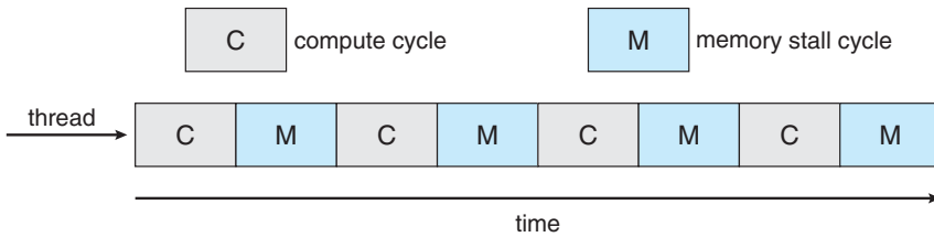
Figure 6.10 Memory stall.
