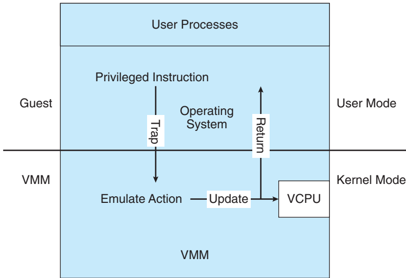
Figure 16.2 Trap-and-emulate virtualization implementation.
